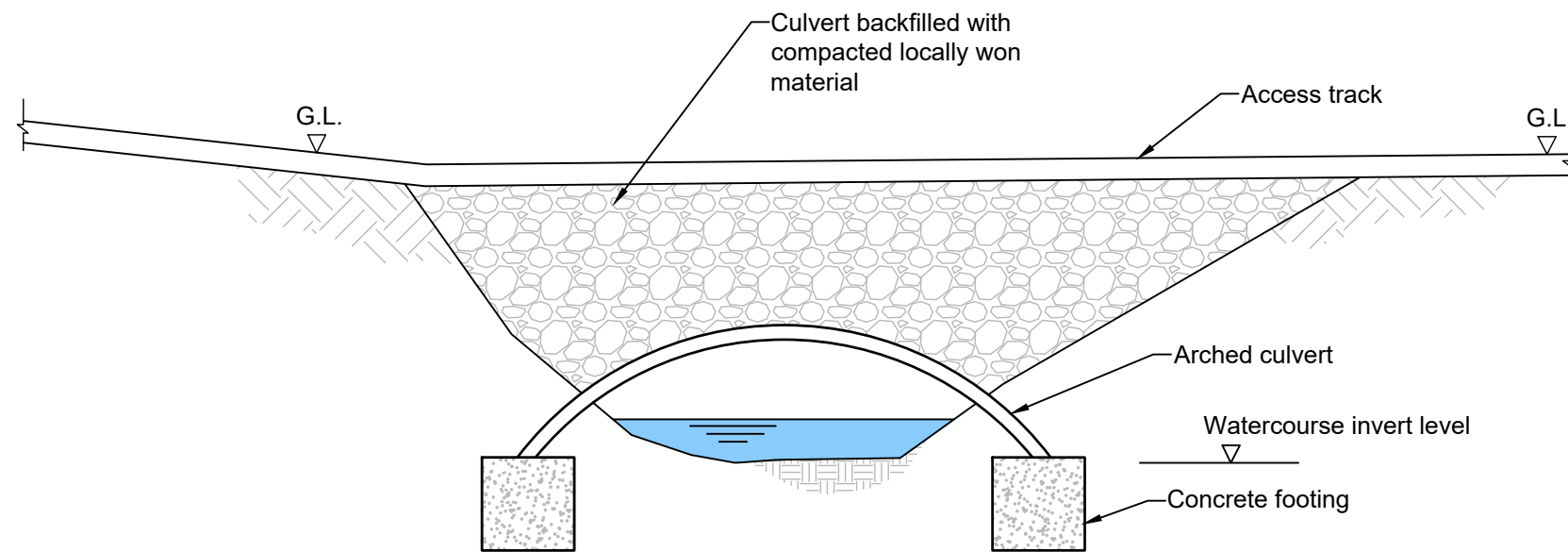
Indicative Bottomless Arched Culvert
